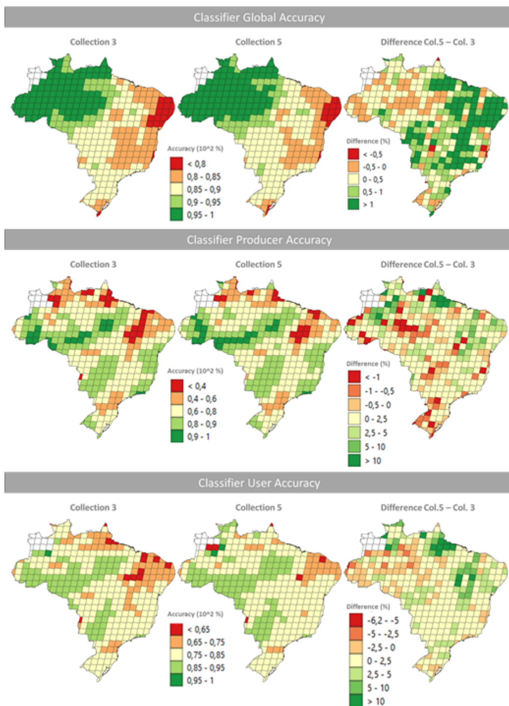
Figure 6. Comparison between the classifier accuracies (scene by scene) reached by the metrics of Collections 3 and 5. The improvements in the classifier performance and capacity to map pasture using the metrics utilized in Collection 5 was significant when compared with Collection 3.
