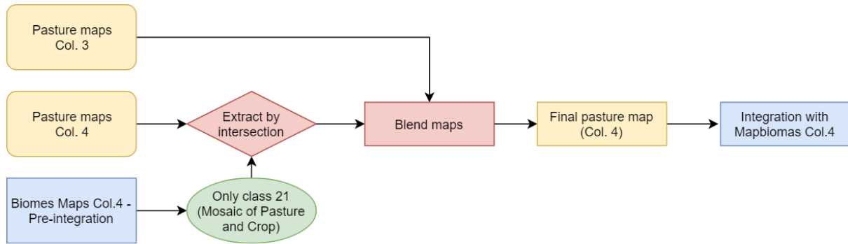
Figure 25. Integration scheme of pasture maps produced in Collection 4.
