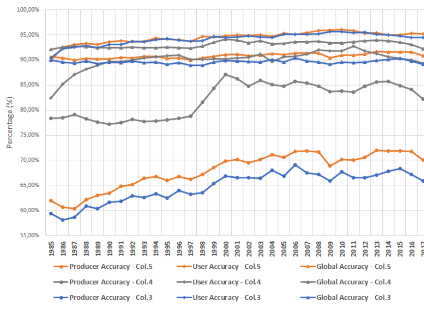
Figure 13. Accuracy assessment results for all the years (and Collections), calculated based on the validation samples, only considering points with four or more votes ( i.e. at least four interpreters identified the same land cover and land use class).
