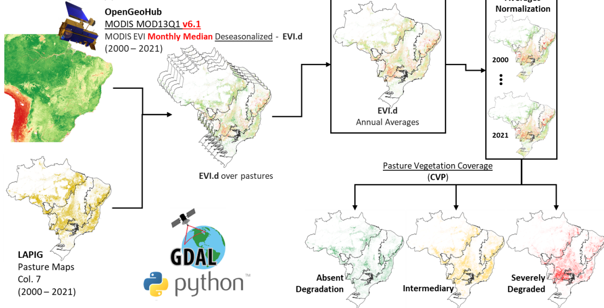
Figure 27. Analysis approach for mapping the quality of the Brazilian pasturelands for Collection 7.
