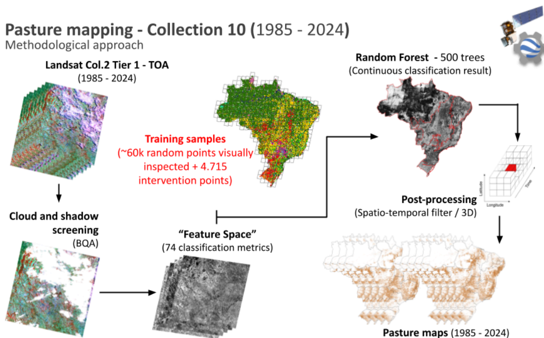
Figure 1. Pasture mapping workflow regarding the MapBiomass Collection 10.
