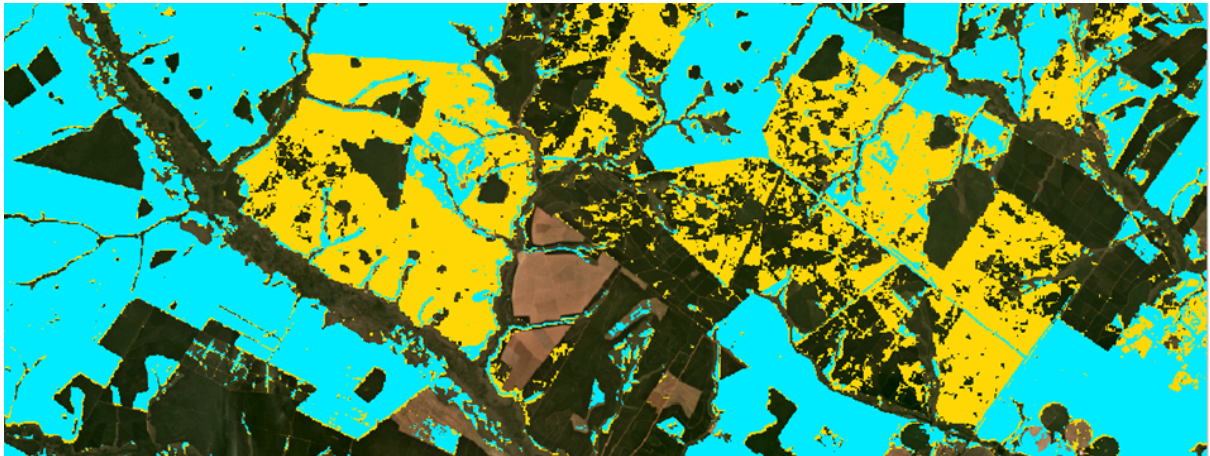
Figure 16. Mapping examples of pasture areas, for the municipality of Brasilândia/Mato Grosso do Sul, in Collections 3 (yellow) and 5 (cyan). In some cases, Collection 3 misclassified planted forest as pasture (since after the cut, grass can grow over these areas).
