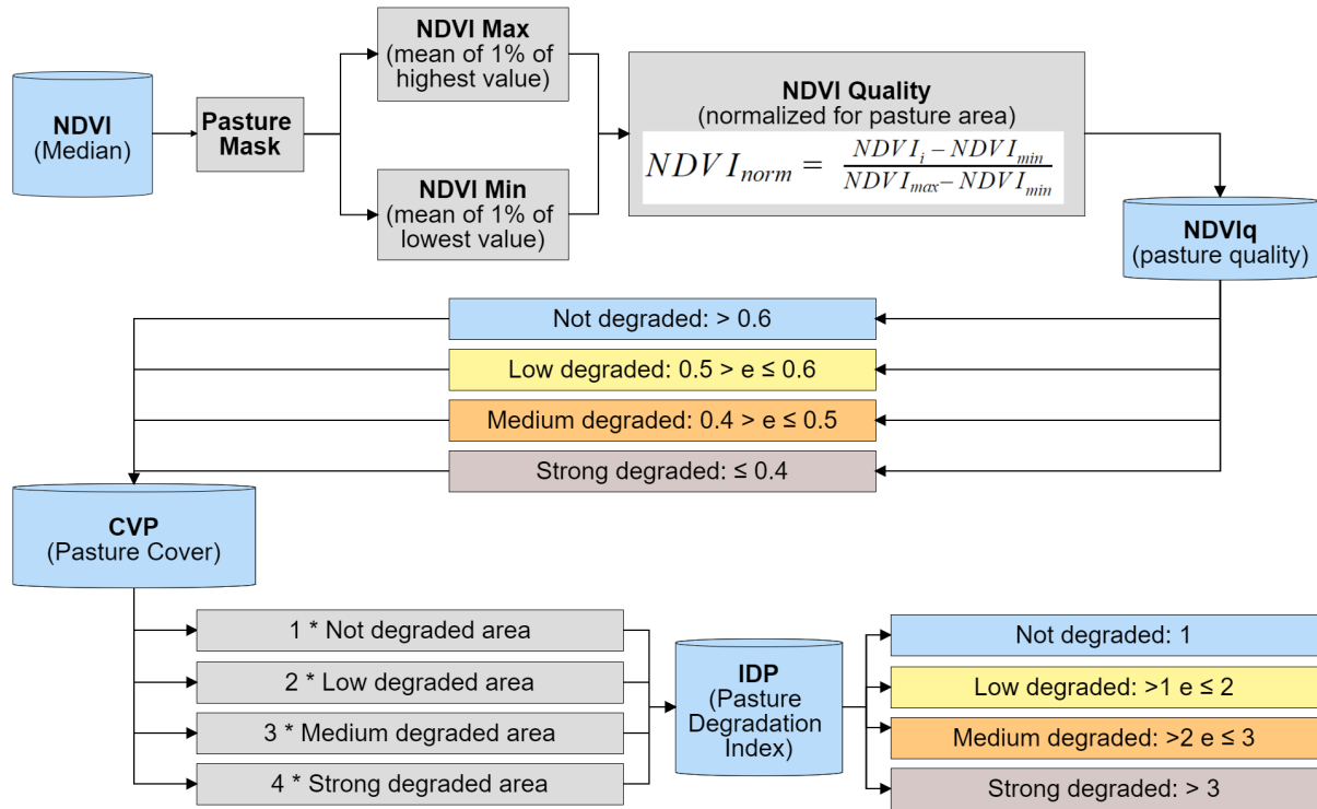
Figure 26. Analysis approach for mapping the quality of the Brazilian pasturelands for Collection 5.
