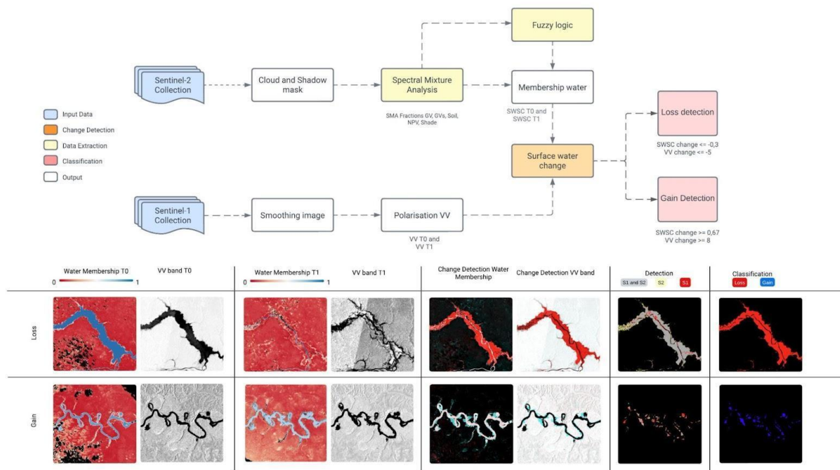
Figure 4. Remote sensing workflow to detect surface water change between 2022 and 2023/2024 (i.e., loss and gain) using Sentinel-1 and Sentinel-2 satellite imagery and examples of surface water change detected with both sensors
