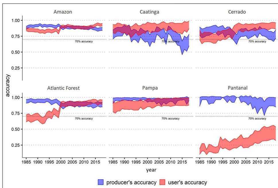
Figure 6. Examples User and producer of “water” class accuracy per biome and per year.
