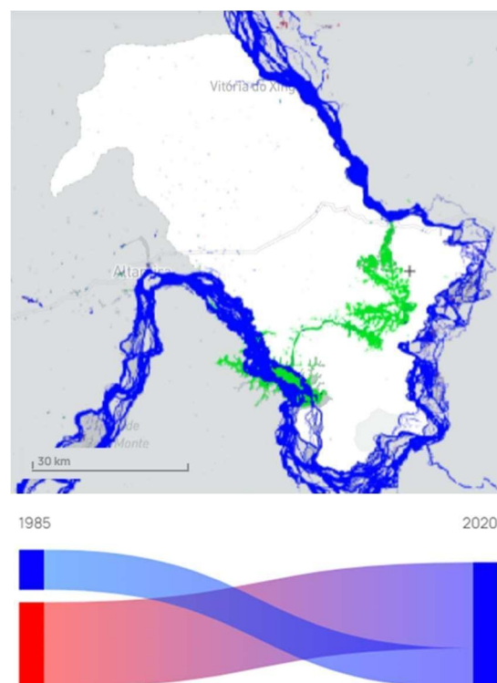
Figure 9. Example of surface water transitions for the Vitória do Xingu municipality. The green in the map indicates the surface water that appeared in the last years with the construction of the Belo Monte dam. A graph (red and blue) indicates the transition between the selected years, according to the mapped water surface area.
