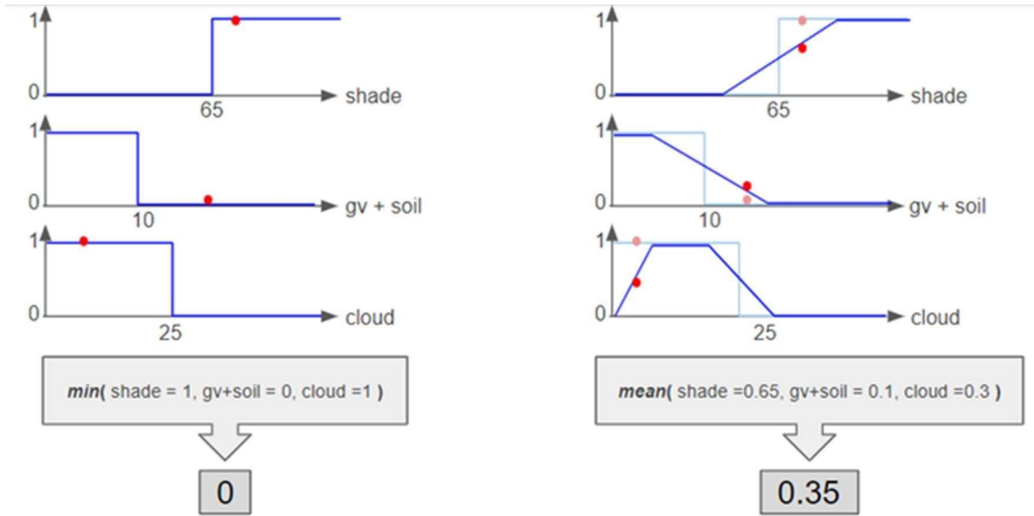
Figure 2. Surface Water Sub-pixel Classifier binary rules. The left example shows an example of undetected surface water for a pixel with fraction values indicated by the red points (the value of gv + soil is above the threshold > 10 to be classified as water). The right example applies a linear probability function to the variable and the mean value allows to correctly classify the pixel (red point) as surface water.
