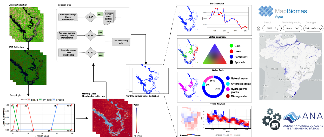
Figure 1. Methodological steps to produce the Brazilian Surface Water Dataset (BSWD), 1985-2024.
