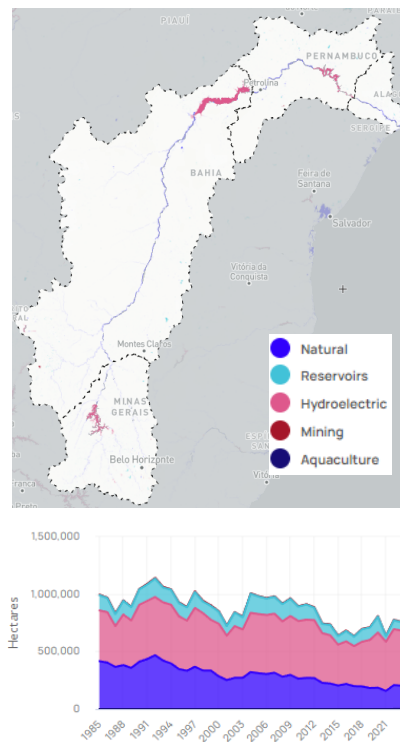
Figure 13. Example of water bodies classification for the São Francisco hydrographic region. The map shows hydroelectrics interrupting the natural water flux of the river in three different sectors. The graph shows the area mapped as surface water among the different classes of water bodies.
