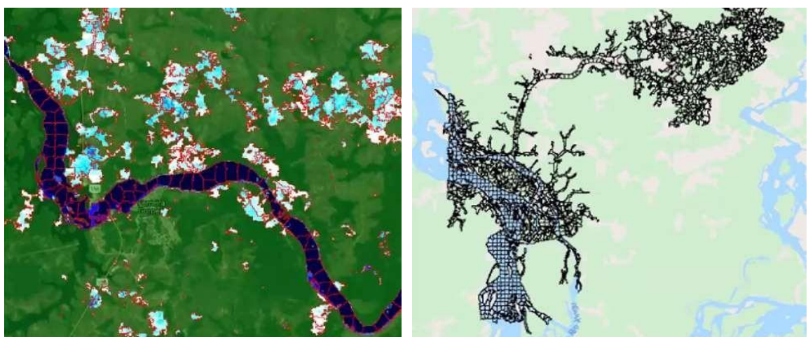
Figure 5. Examples of the segmentation process converting raster data (monthly frequency within each year) into a fishnet of regular vectors.
