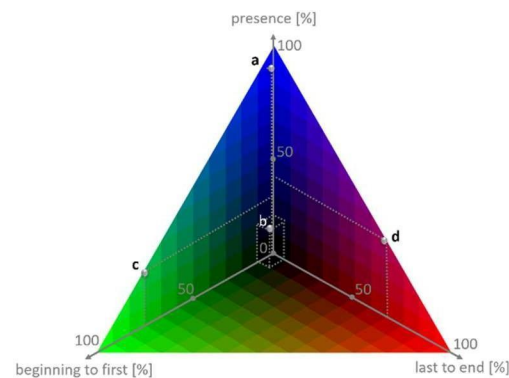
Figure 8. RGB surface water dynamics. Blue colors indicate persistence, as the total number of years classified as surface water; green appearance (the number of years from the beginning of the time-series until the first classification); and red disappearance. Black and dark colors indicate sporadic or non-permanent surface water.
