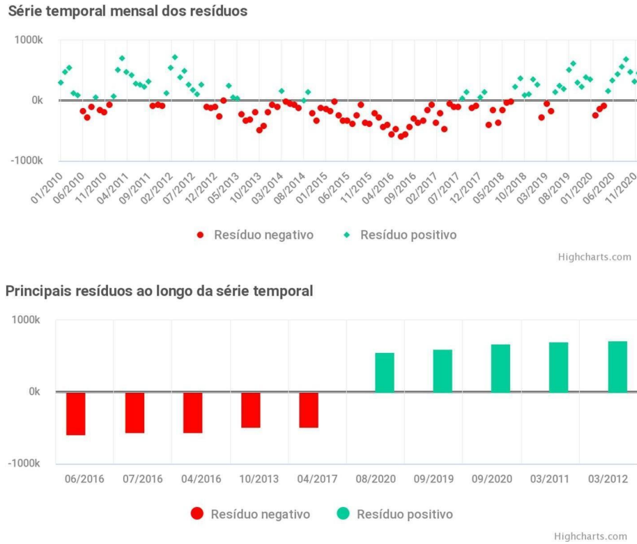
Figure 11. Example of differences between the fitted model and observed data. Green points and bars indicate increased values, red points and bars indicate decreased values in relation to the expected by the harmonic model.
