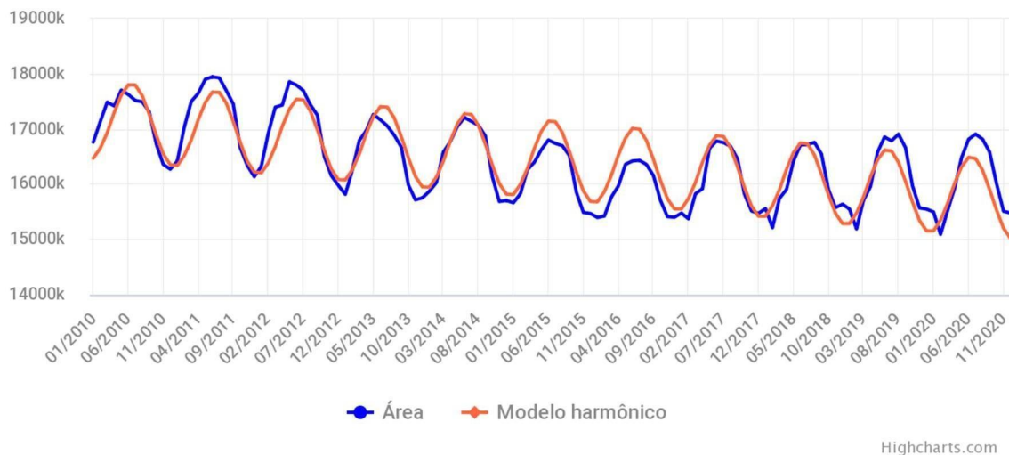
Figure 10. Example of fitting a harmonic series to the results of mapped monthly water surface data. The blue line is the mapped water surface area, the red line indicates the harmonic fitted model.
