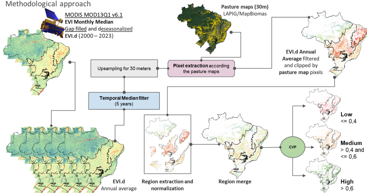
Figure 28. Analysis approach for mapping the vigor of the Brazilian pasturelands for Collection 9.
