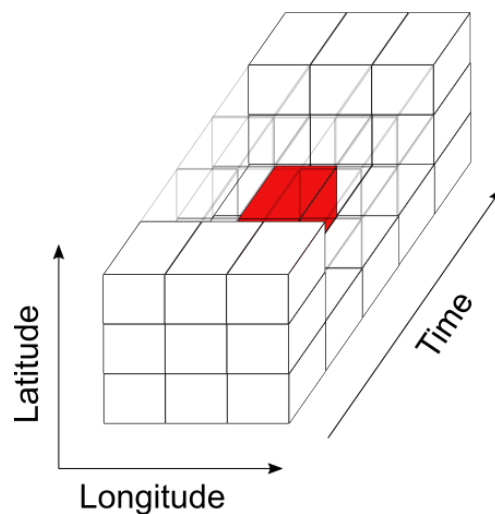
Figure 9. The kernel, with 3x3 pixels and 5 years, used in the space-time filtering of the probability pasture maps produced with Random Forest. The central pixel, highlighted in red, is replaced by the median of the probabilities of the 45 pixels kernel.
