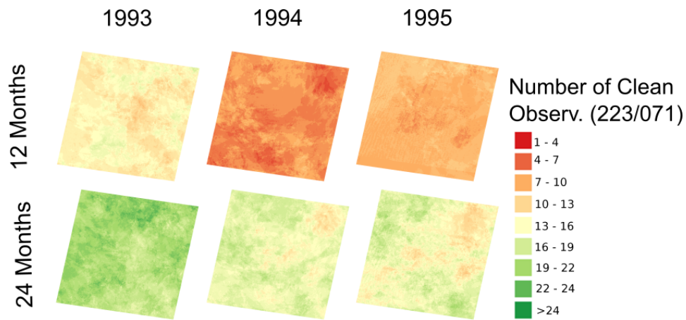
Figure 2. Number of clean observations (without clouds and cloud shadows) available for the Landsat scene 223/071, considering 12 months ( i.e. without year overlap) and 24 months ( i.e. the 1994 image considered observations of the second half of 1993 and the first half of 1995).
