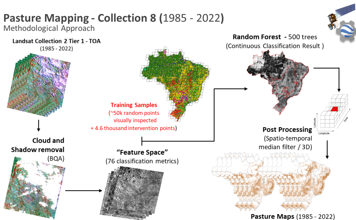
Figure 1. Pasture mapping workflow regarding the MapBiomass Collection 7.
