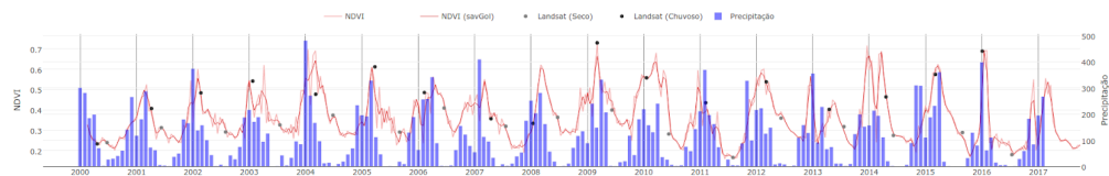
Figure 5. Temporal Visual Inspection tool (TVI) which allows the users to visualize two Landsat images, regarding the dry and wet seasons, as well a MOD13Q1 NDVI time series. This image is located in Luís Eduardo Magalhães - BA.
