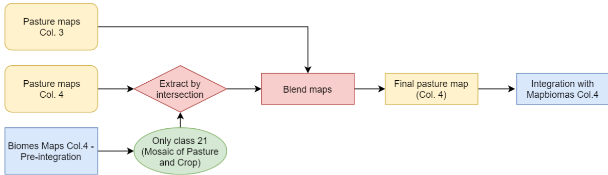
Figure 20. Integration scheme of pasture maps produced in Collection 4.
