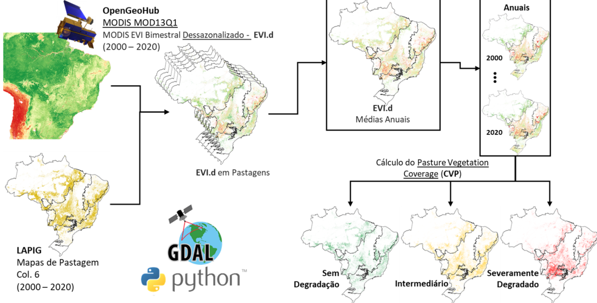
Figure 22. Analysis approach for mapping the quality of the brazilian pasturelands for Collection 6.
