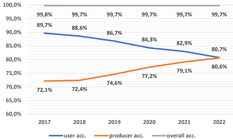
Figure 5. Accuracy results by year in collection 3
