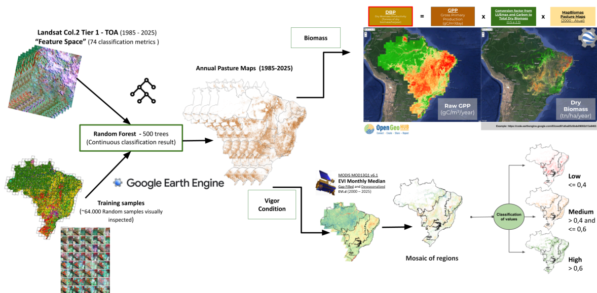
Figure 1. Pasture mapping workflow regarding the MapBiomass Collection 11.
