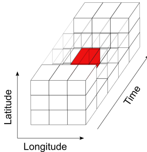
Figure 10. The kernel, with 3x3 pixels and 5 years, is used in the space-time filtering of the probability pasture maps produced with Random Forest. The central pixel, highlighted in red, is replaced by the median of the probabilities of the 45 pixels kernel.
