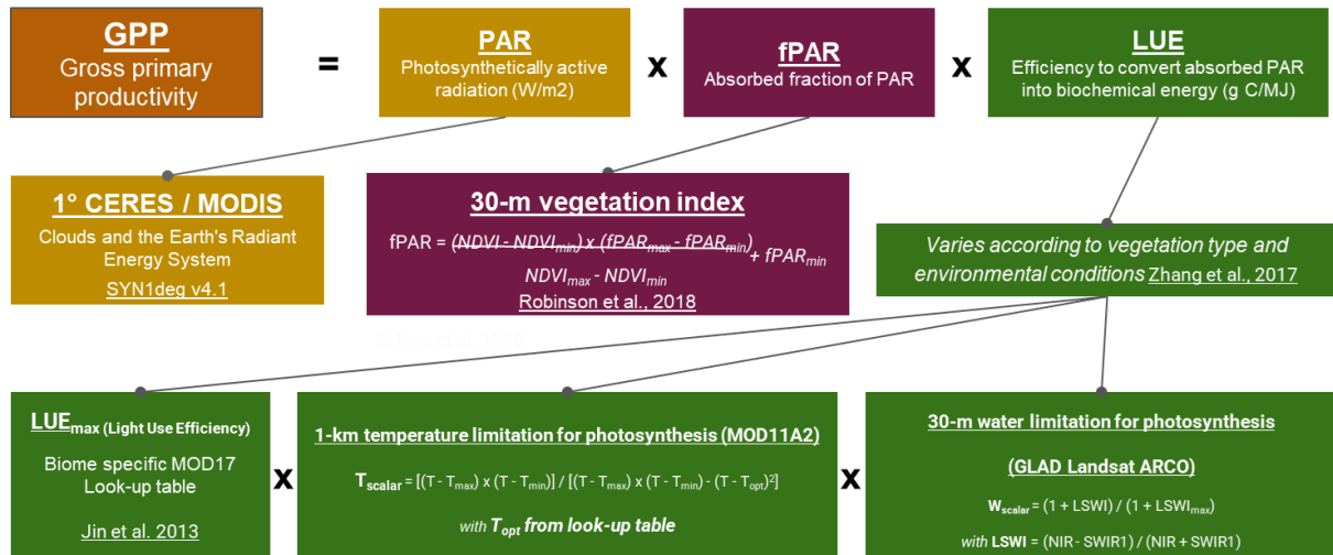
Figure 31. Workflow used to estimate GPP based on Robinson et al. (2018) and Veloso et al. (2020) approaches.
