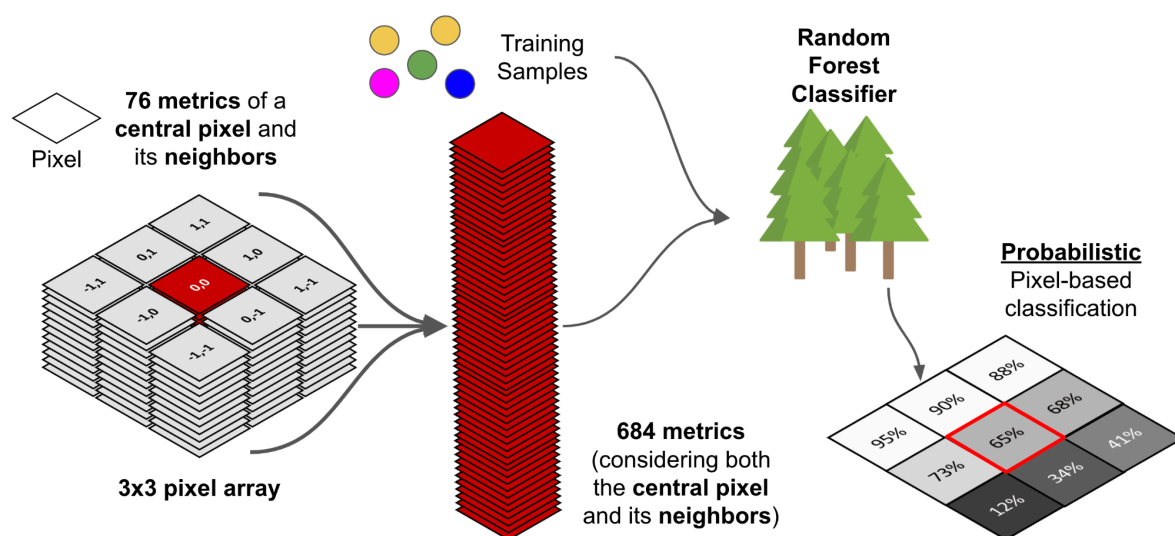
Figure 7. Use of context information evaluated in Collection 7.
