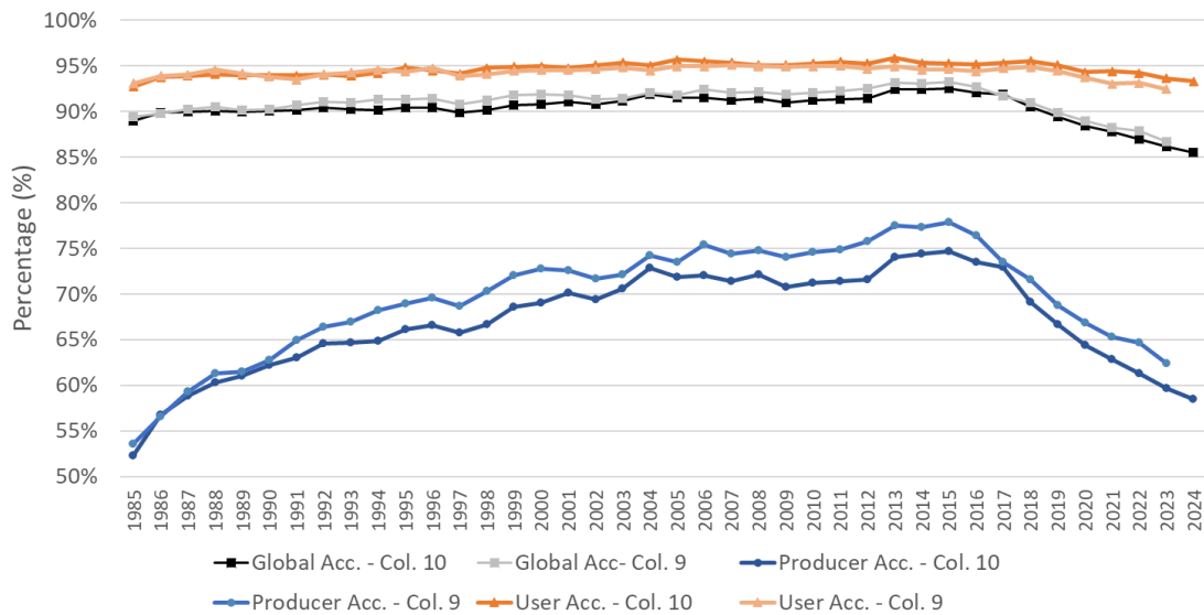
Figure 23. Accuracy assessment (on an annual basis) for Collections 9 and 10, calculated based on the validation samples, only considering points with four or more votes ( i.e. at least four interpreters identified the same land cover and land use class).
