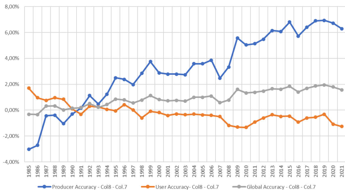
Figure 21. Percentual differences in accuracies between Collections 7 and 8. The revision and increment of new training samples, as well as the usage of intervention training points, helped to boost the accuracy values in Collection 8 (at the cost of slightly decreasing the user accuracy).
