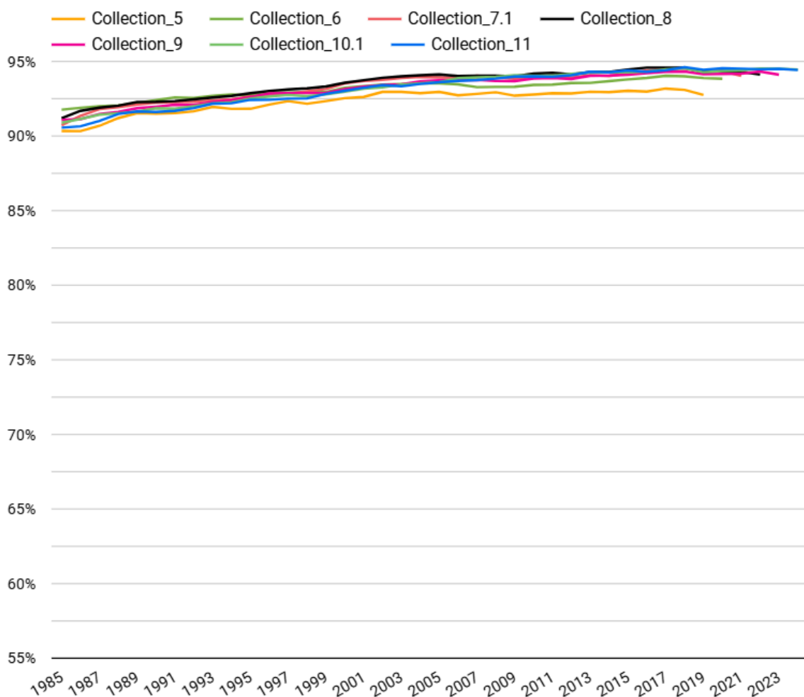
Figure 11. Global accuracy for Atlantic Forest biome at legend level 1.
