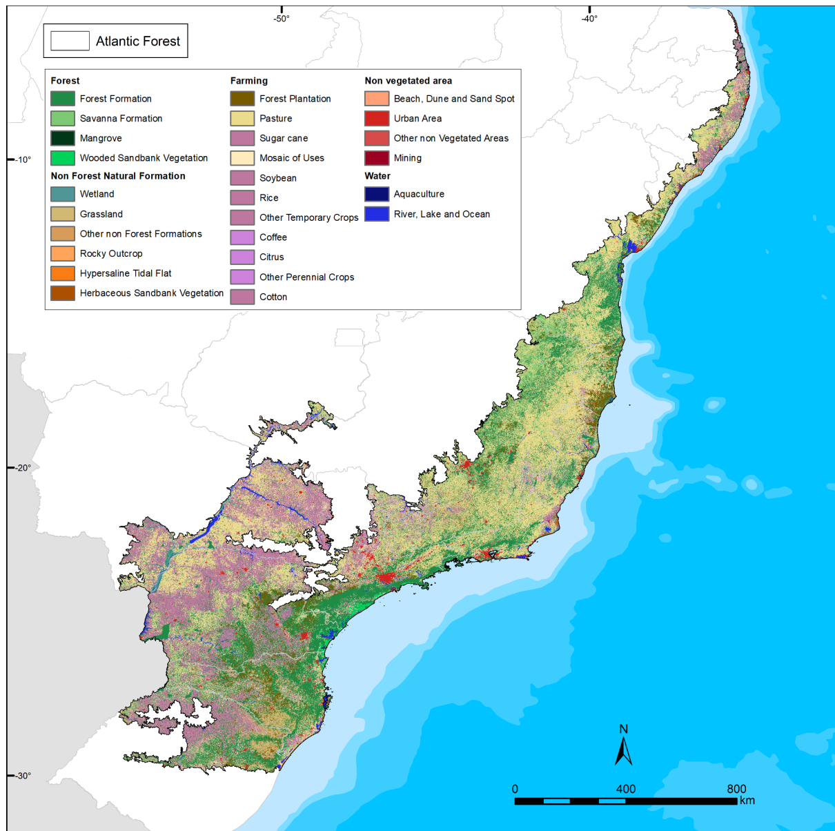
Figure 9. Final land use and land cover map of the Atlantic Forest biome - 2025
